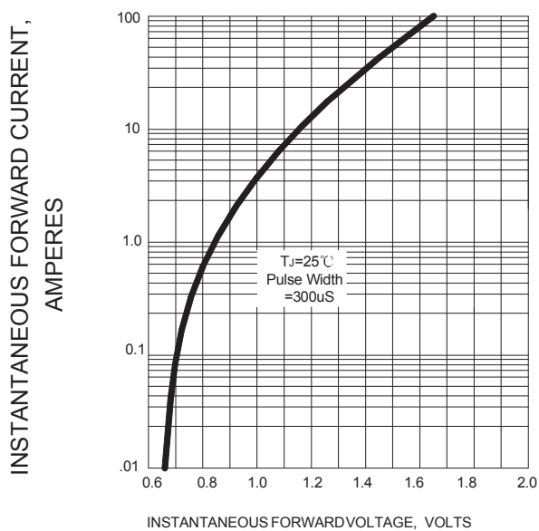
FIG.3 – TYPICAL FORWARD CHARACTERISTIC
