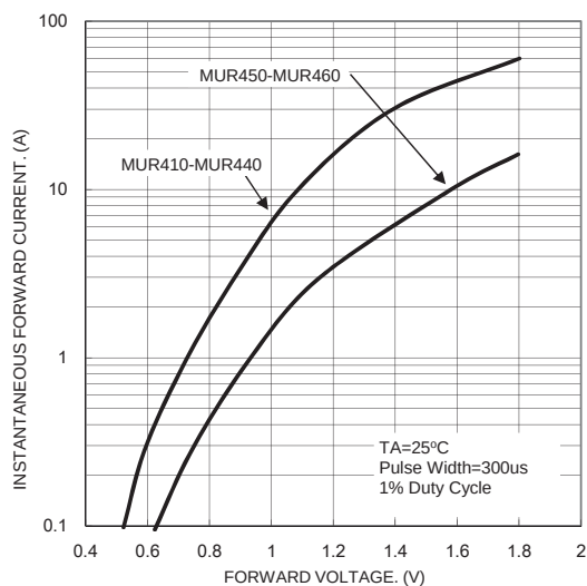
FIG. 5-TYPICAL FORWARD CHARACTERISTICS
