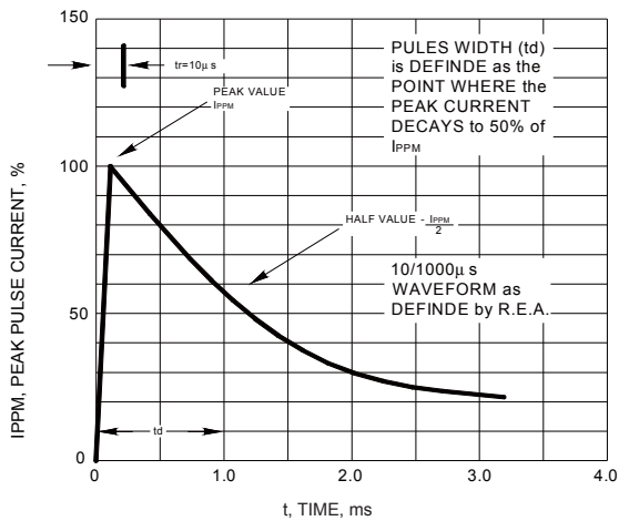
FIG.3 -- PULSE WAVEFORM
