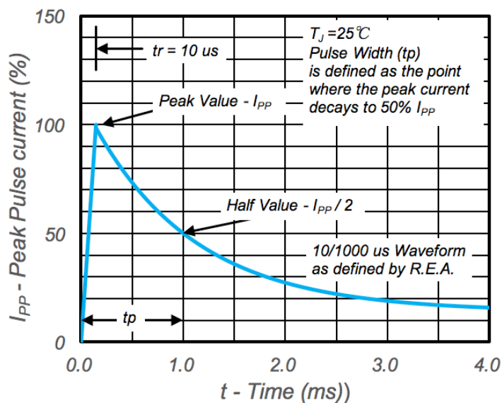
Fig.3 - Pulse Waveform
